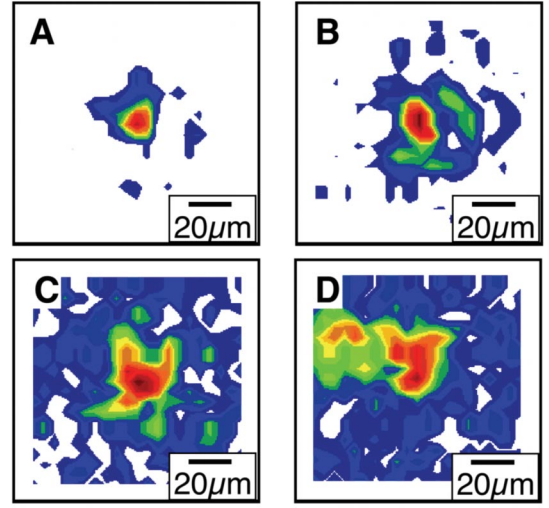
FIG. 4 (color). Channel tuning to compensate for self-guiding. The effect of self-guiding on mode structure is shown by varying the input power in a channel tuned to guide low intensity pulses. For pulses at 0.5 TW, below the critical power for self-guiding, the output mode is undistorted (a). As power is increased to 2 TW (b), some distortion is evident and this becomes more severe as power is further increased to 4 TW (c) and 8 TW (d). Guides were tuned to guide modes up to 4 TW without distortion by adjusting the density profile to compensate for self-guiding (Fig. 3).
